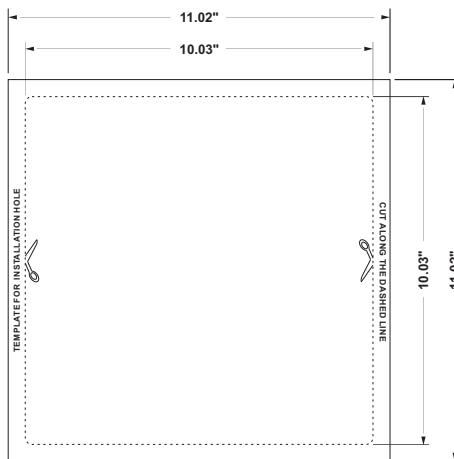
Dimensions for ceiling cutting
